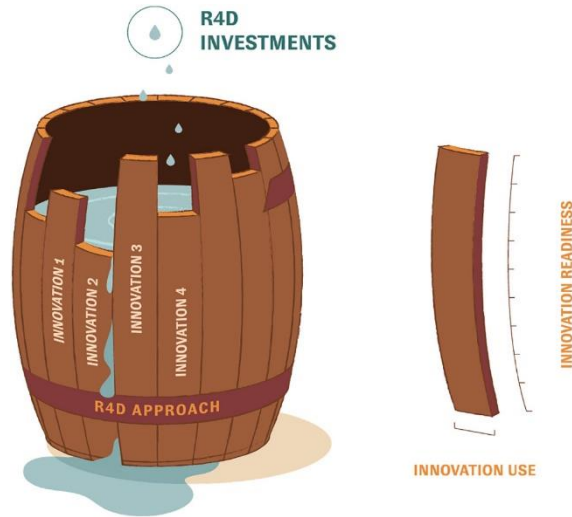
Scaling Readiness
