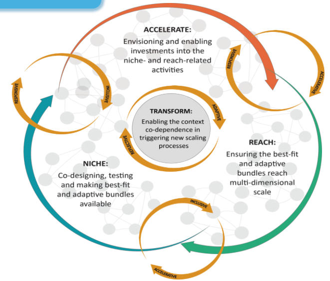
Adaptive scaling
